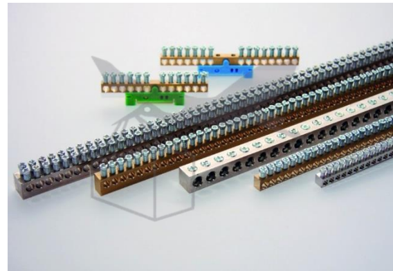
BRASS TERMINALS
